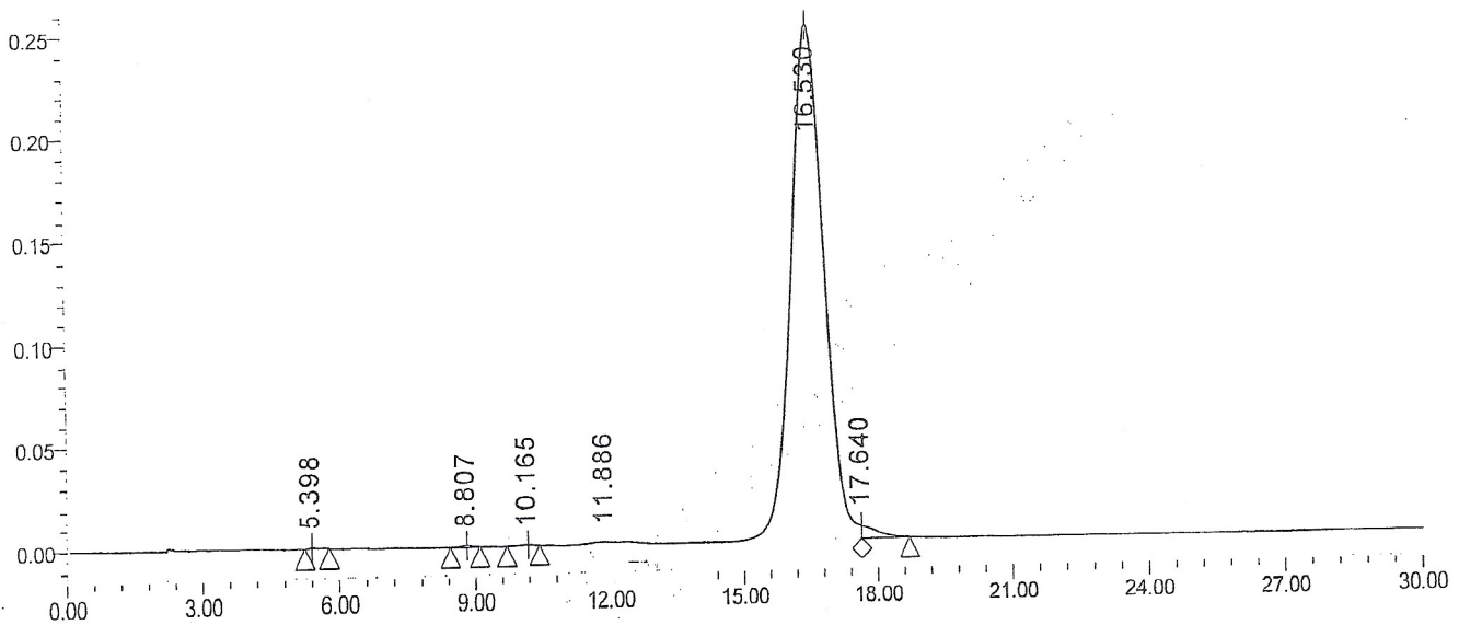
Auto-Scaled Chromatogram
